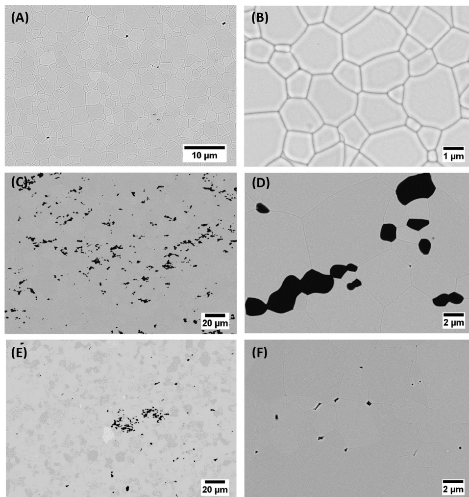
FIGURE 2 Secondary electron scanning electron microscopy (SEM) images of samples after sintering. (A, B) Yttrium aluminum garnet (YAG). (C, D) Erbium aluminum garnet (ErAG). (E, F) Lutetium aluminum garnet (LuAG).
