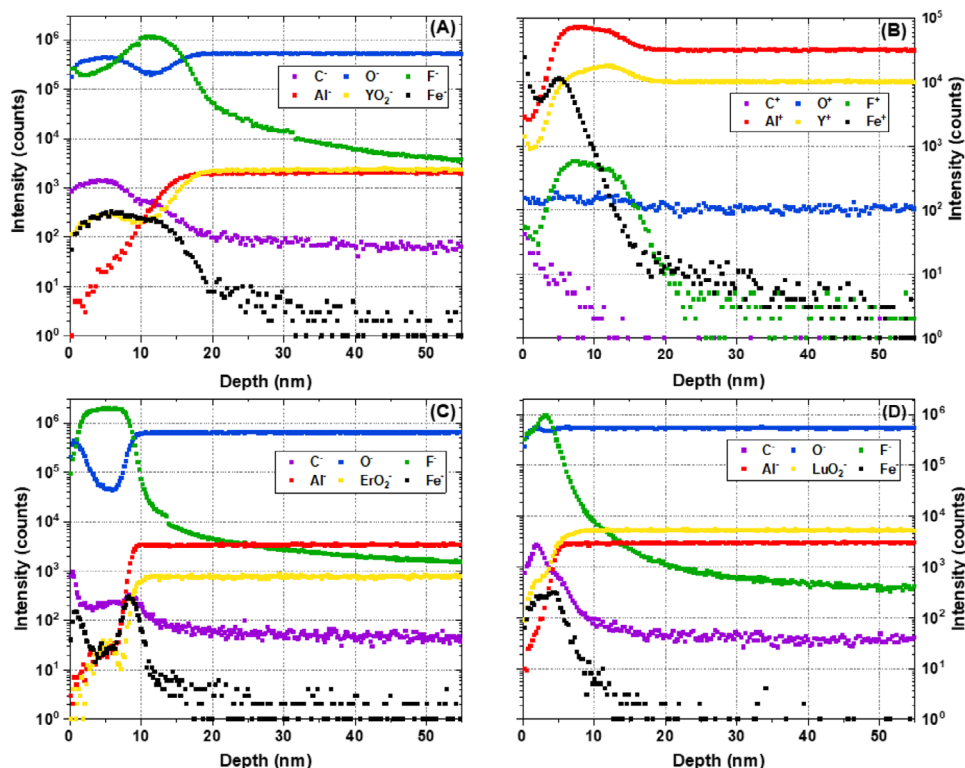
FIGURE 4 Time-of-flight secondary ion mass spectrometry (ToF-SIMS) depth profiles of all samples after plasma etching. (A) Yttrium aluminum garnet (YAG; negative polarity). (B) YAG (positive polarity). (C) Erbium aluminum garnet (ErAG; negative polarity). (D) Lutetium aluminum garnet (LuAG; negative polarity).
